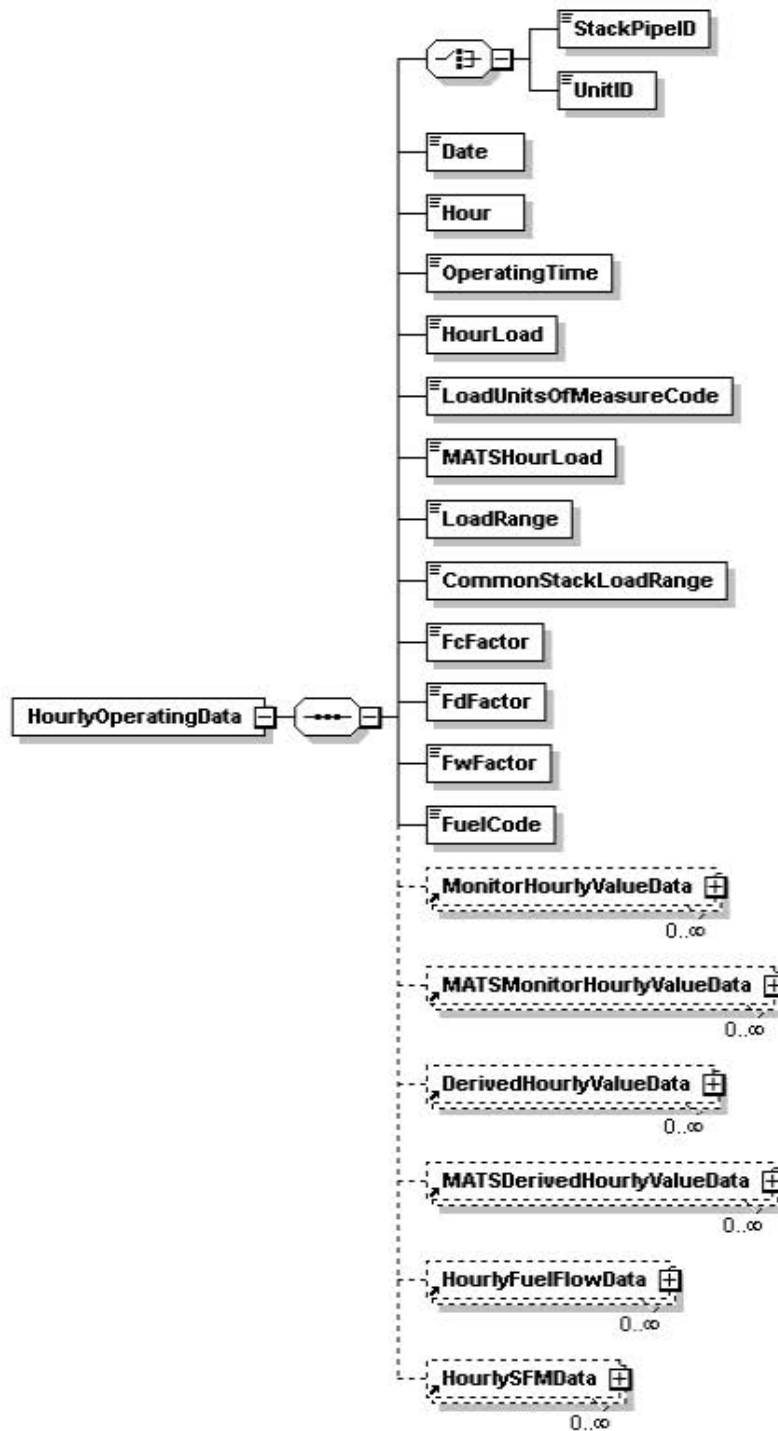
Figure 10 HOURLY OPERATING DATA XML Elements
