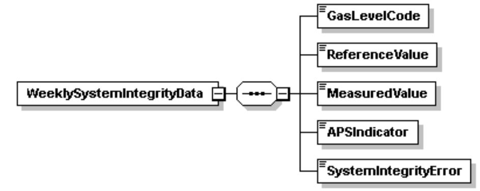
Figure 7 WEEKLY SYSTEM INTEGRITY DATA XML Elements
