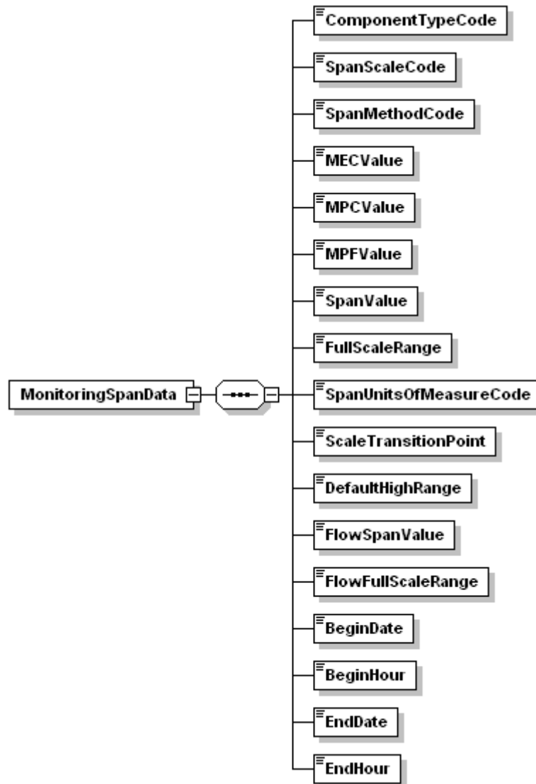
Figure 20-21 MONITORING SPAN DATA XML Elements
