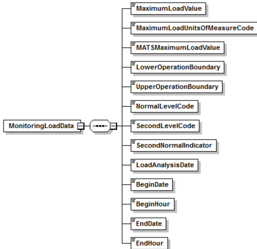
Figure 22-23 MONITORING LOAD DATA XML Elements
